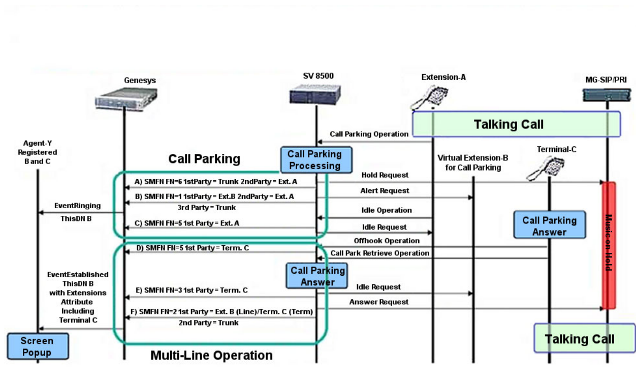
Figure 14: Call Parking
