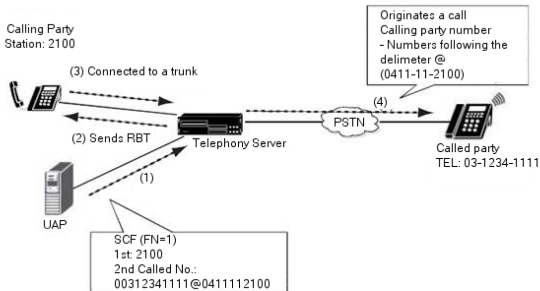
Figure 17: Using the Called Number Parameter in the SCF Request
