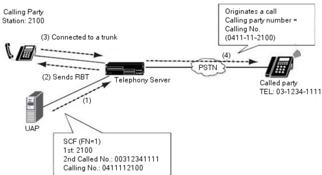
Figure 18: Using the Called Number Information in the SCF OAI Request
