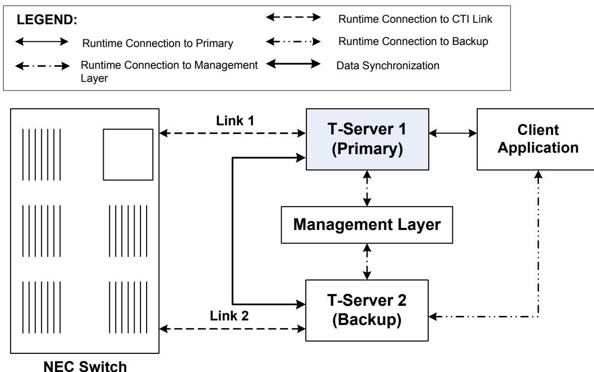
Figure 13: Warm and Hot Standby T-Server Configuration
